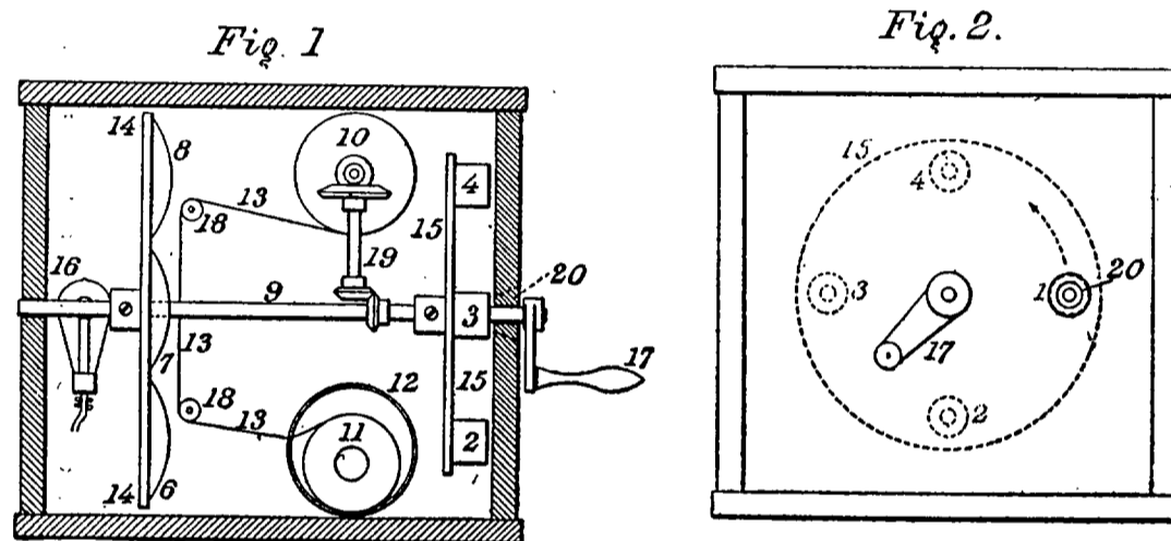
JENKINS' ROTARY LENS CAMERA.
